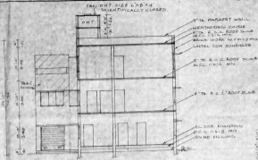
SECTION ON 50'
