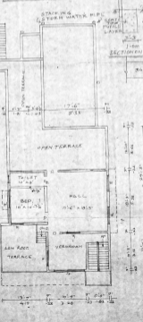
PROPOSED SECOND FLOOR PLAN
